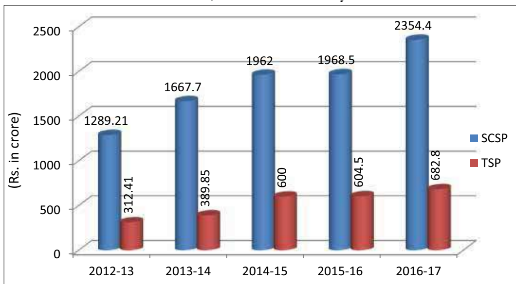
Figure 4.13 SCSP/TSP-Yearwise Outlay
